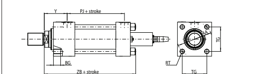
Z (ISO MX5) = front threaded holes
