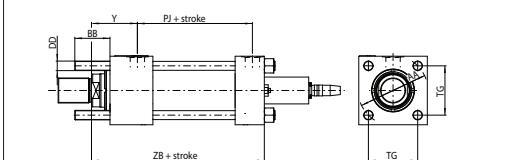
Y (ISO MX3) = front tie rods extended
