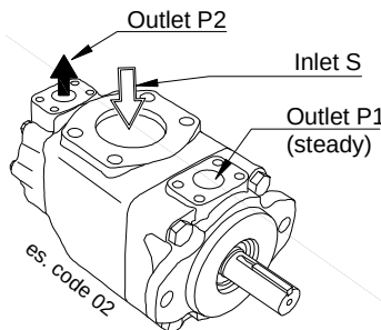
Port orientations
