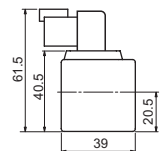
"CX" Deutsch with diode
