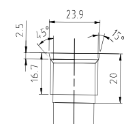
SAE O-Ring Port 10 thread ANSI B1.1 1 7/8 UN-2B
