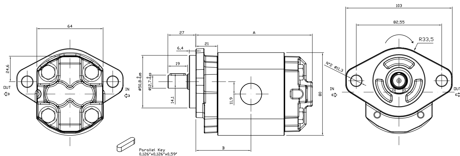
GR28 - TYPE / TIPO SAE A-A SAE O-RING PORT 3/4 14 UNF 2B
