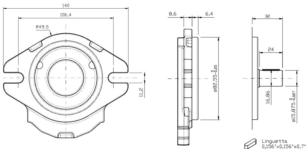
GR38 - TYPE / TIPO SAEA-AC SAE O-RING PORT UNF
