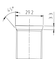
SAE O-Ring Port 12 thread ANSI B1.1 1 1/16 UN-2B
