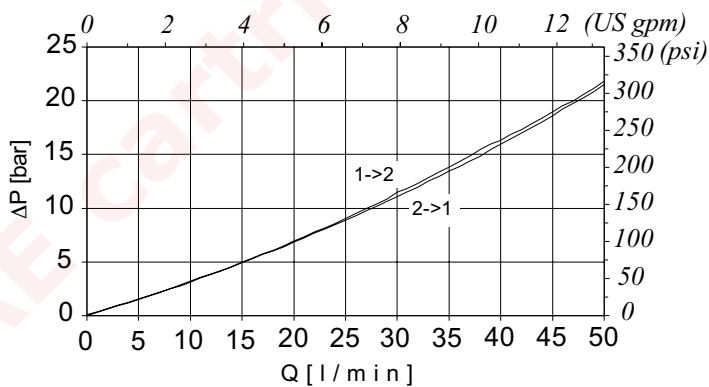
Typical pressure drop vs. flow characteristics Oil viscosity 46 cst at 40°
