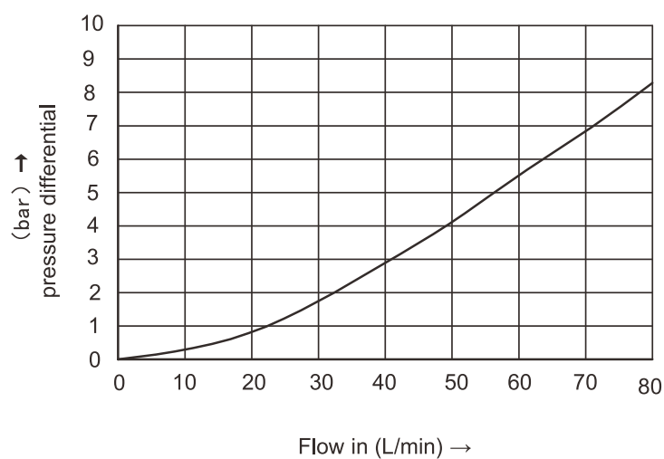
\Delta p-q_v Characteristic curves
