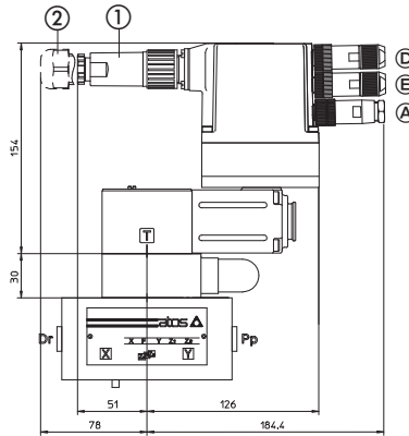
LI*ZO-AES-EH-4...6/**/P
