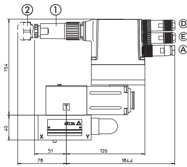
LI*ZO-AES-EH-1...3
