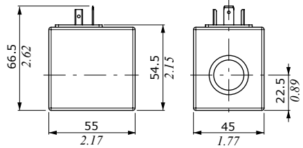
ISO4400 connector
