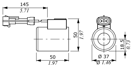
Flying leads with PACKARD METRI-PACK connector
