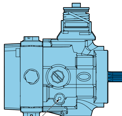
Setting screw
