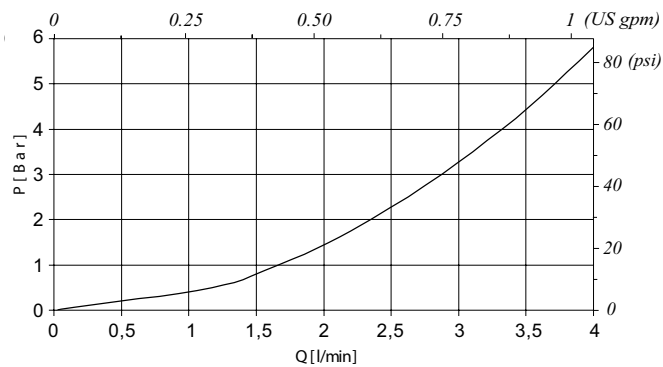
Typical Pressure drop vs. flow characteristic 1 → 3 with de-energized coil Oil viscosity 46j cSt at 40j C
