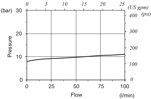
Pressure drop from P to C (referred to SDS140/1)
