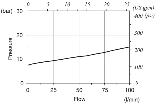
Pressure drop P to T (referred to SDS140/1)
