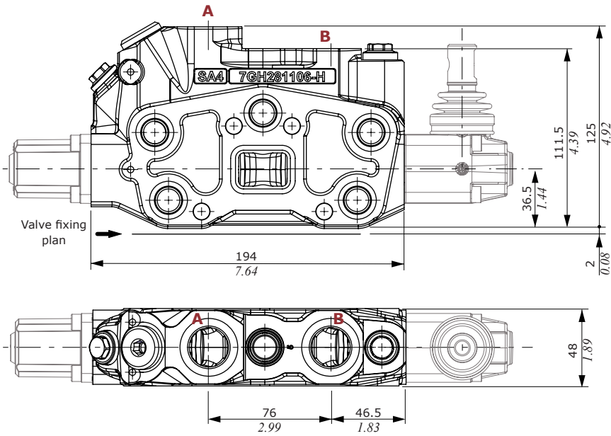
RPH5LL type
