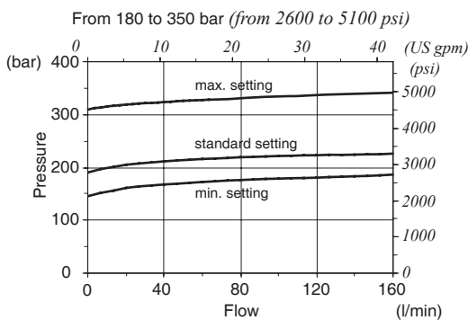
G4 setting range
