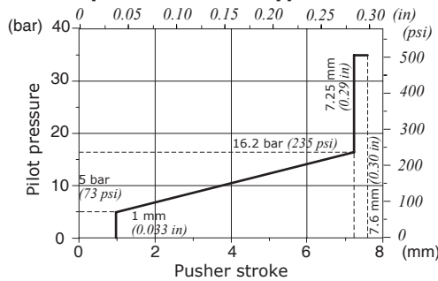
Pressure control curve on port VA and VB: type 075
