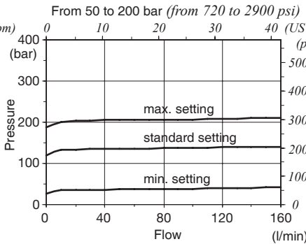
LSW(G3) main relief valve setting range
