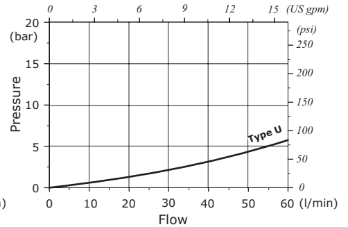
Pressure drop (in anticavitation)
