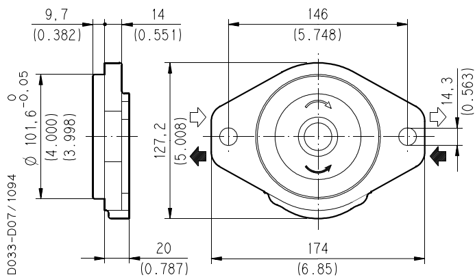
SAE "B" 2 BOLT
