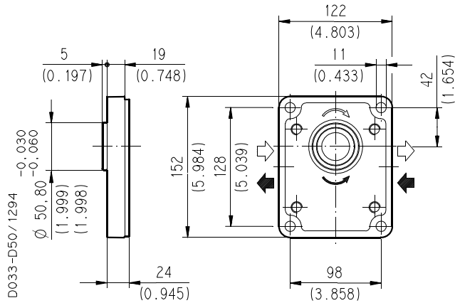
GERMAN RECTANGULAR B3
