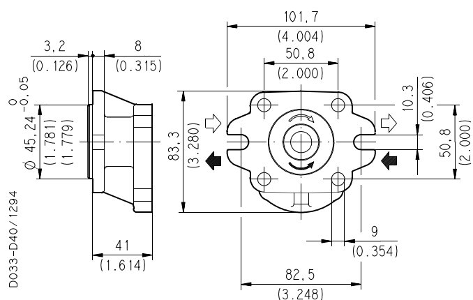
SAE 2-4 BOLT
