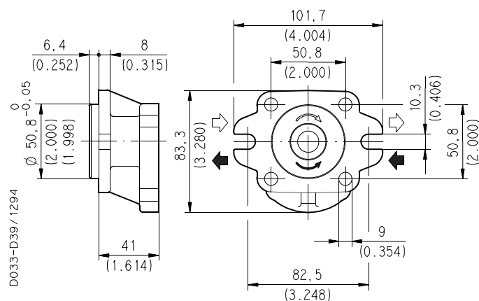
SAE 2-4 BOLT
