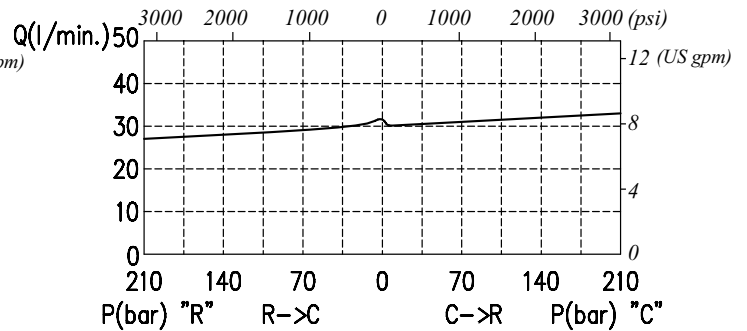
Pressure compensation diagram (12)
