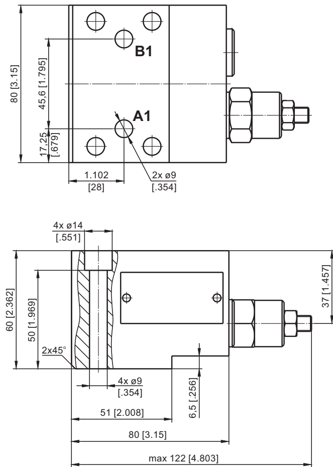
SINGLE VALVE KPBHR-250/1/AE...
