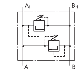
Dual Crossover Relief Valves type KPDHR... and KPDRK...
