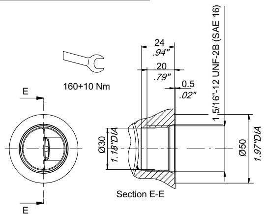
1 5/16" 12 UNF-2B (SAE16)
