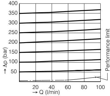
\Delta p -Q for check valve
