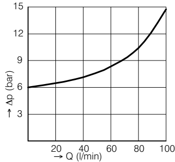
\Delta p -Q for check valve
