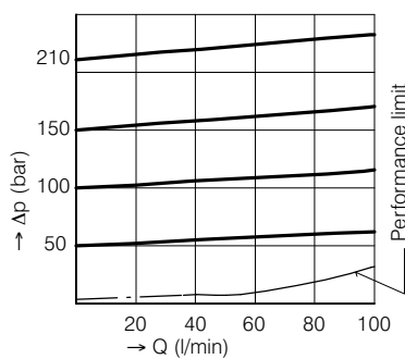
\Delta p -Q characteristic DVPA-RV-1-10-...M
