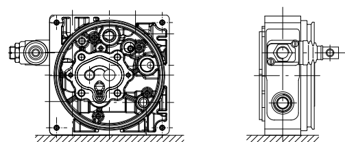
Hand lever
