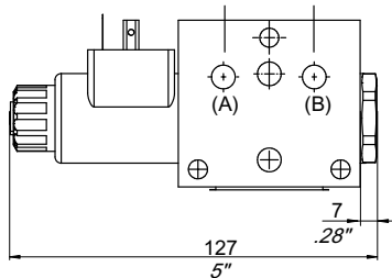
Valve with one solenoid "B" - Circuit: C-01
