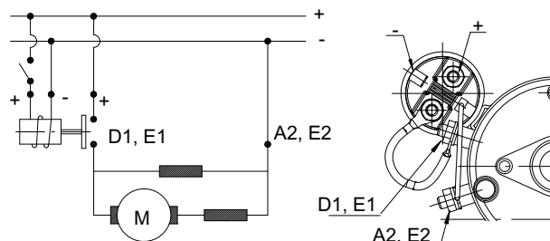
Electric diagram
