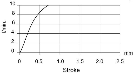
Metering performance.
