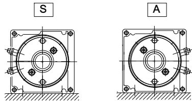
Standard positions
