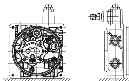
Hand lever
