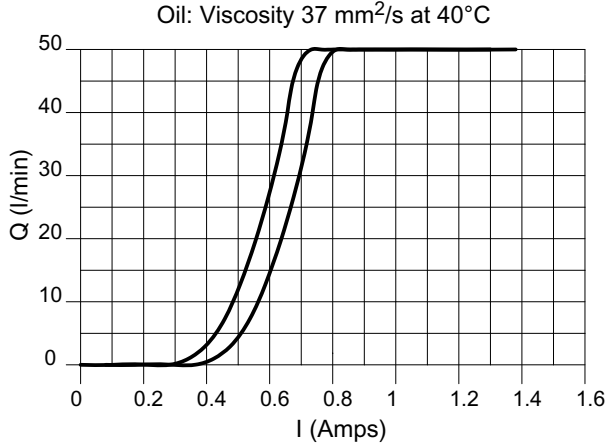
Typical hysteresis
