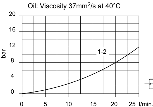
Lever stick
