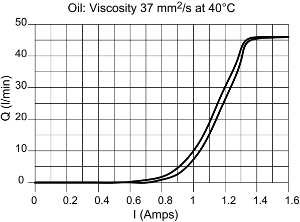
Typical hysteresis
