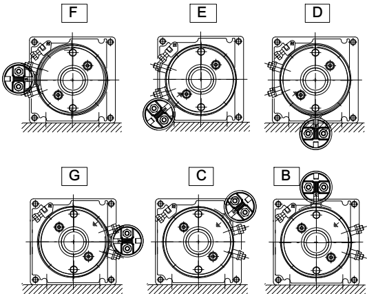
Relay mounting positions
