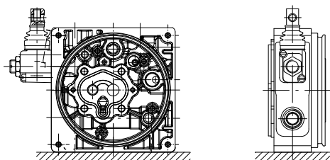
Hand lever
