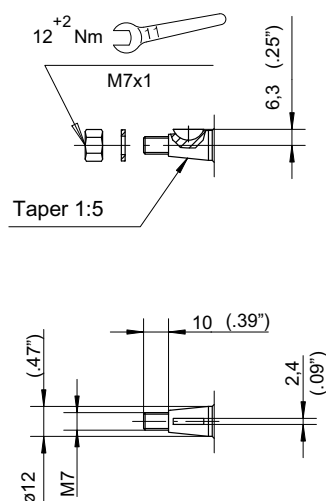
Shaft end
