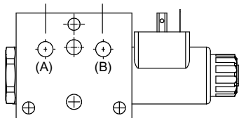
Valve with one solenoid "B" - Circuit: C-01
